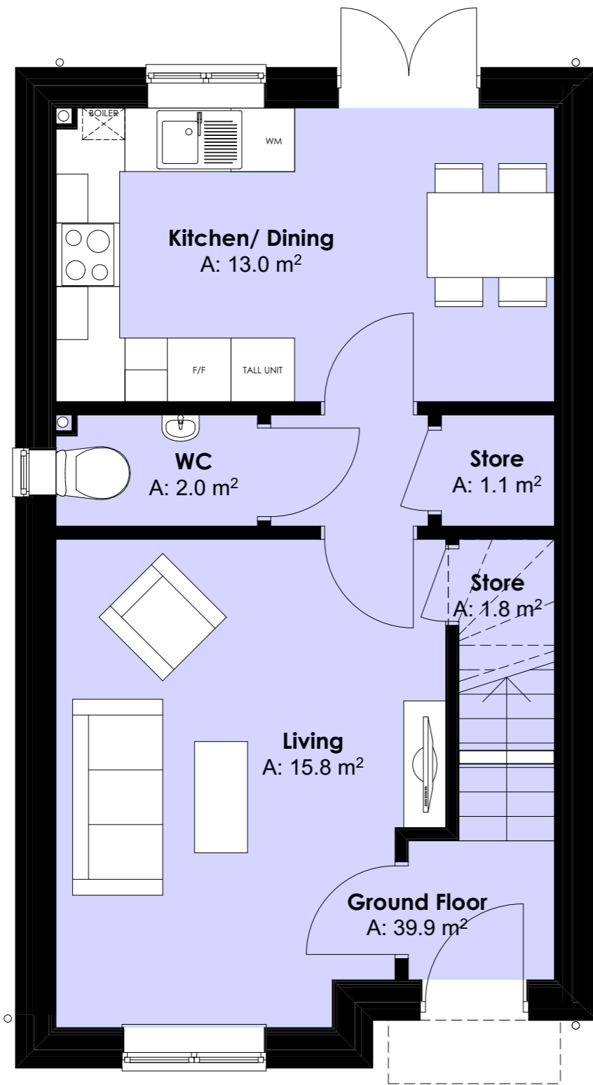
2B4P HOUSE GROUND FLOOR PLAN Total Floor Area: 79.8m 2
