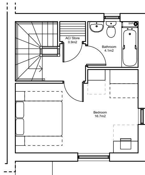
First Floor 1B2P House
