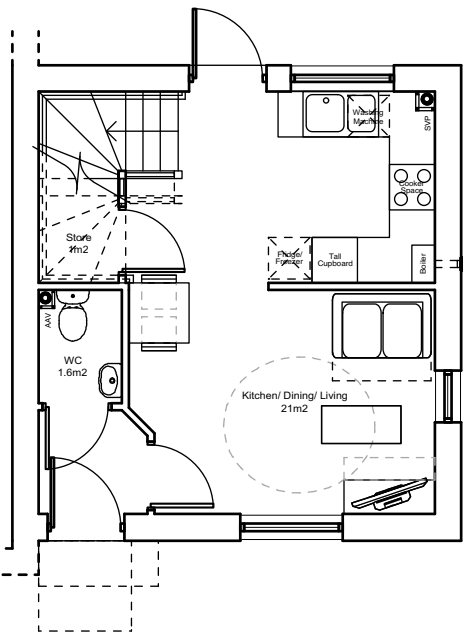
Ground Floor 1B2P House @58.5m 2
