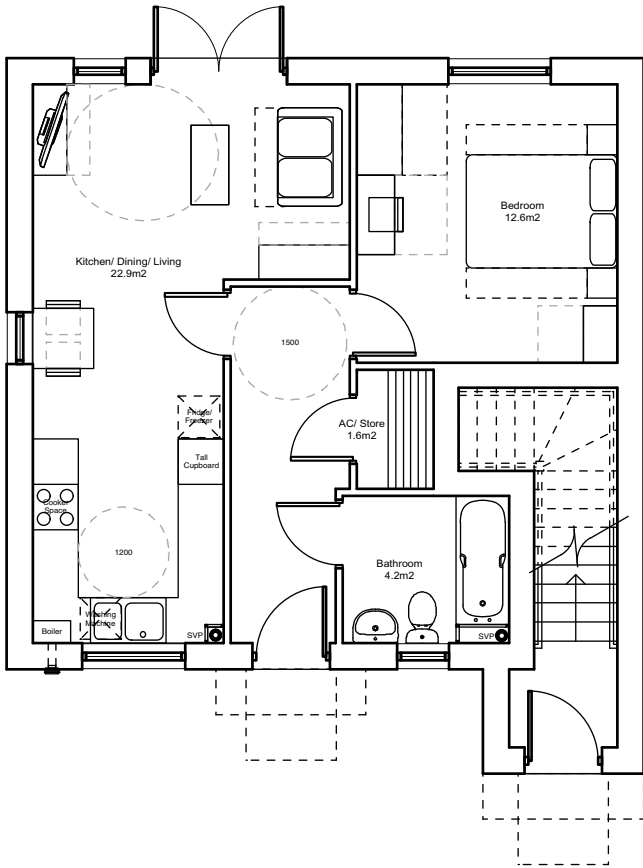
Ground Floor 1B2P Flat @50.0m 2
