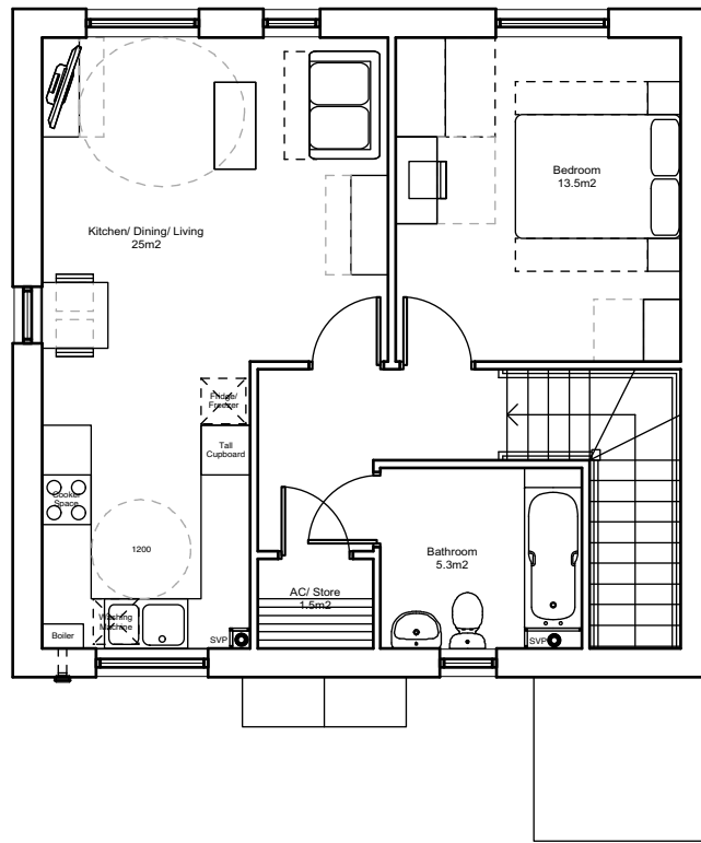
First Floor 1B2P Flat @59m 2
