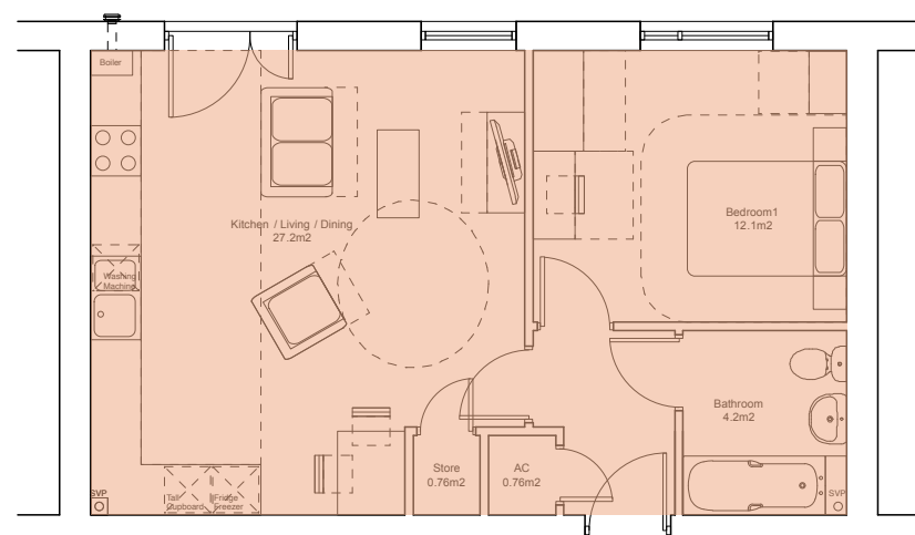
Typical 1B2P Unit Plan (1:100)
