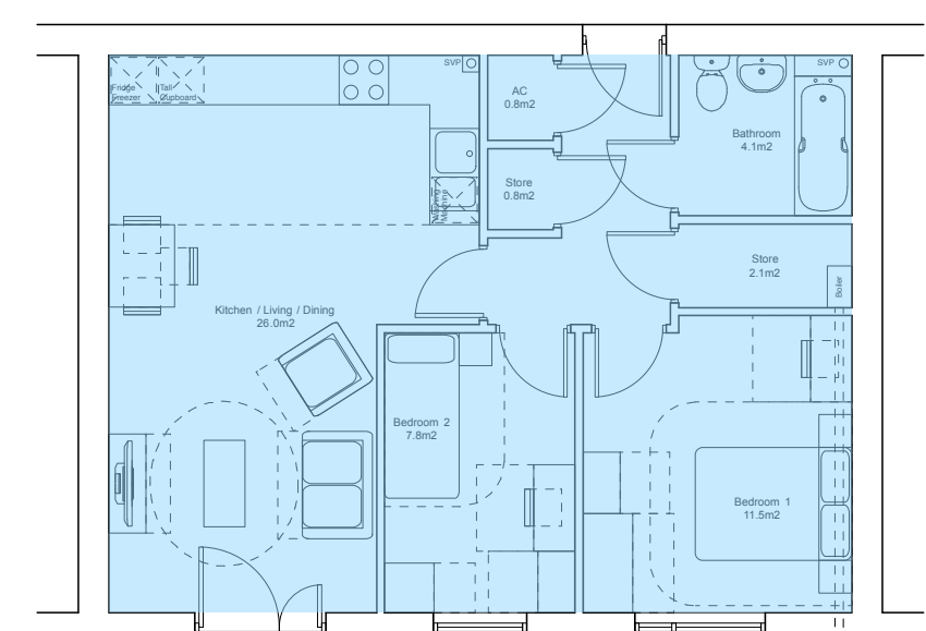
Typical 2B3P Unit Plan (1:100)
